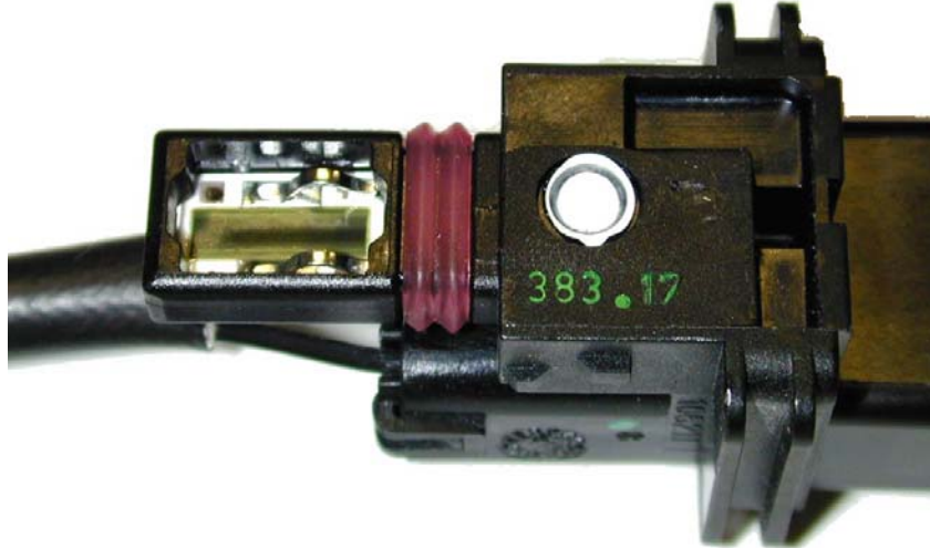
Figure 2. UEGO Sensor laser etched calibration resistor
