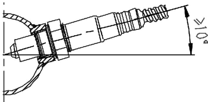
Figure 8. Minimum mounting angle for the UEGO Sensor
